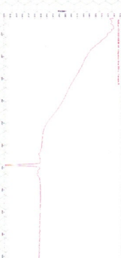
Ultraviolet-visible spectroscopy
